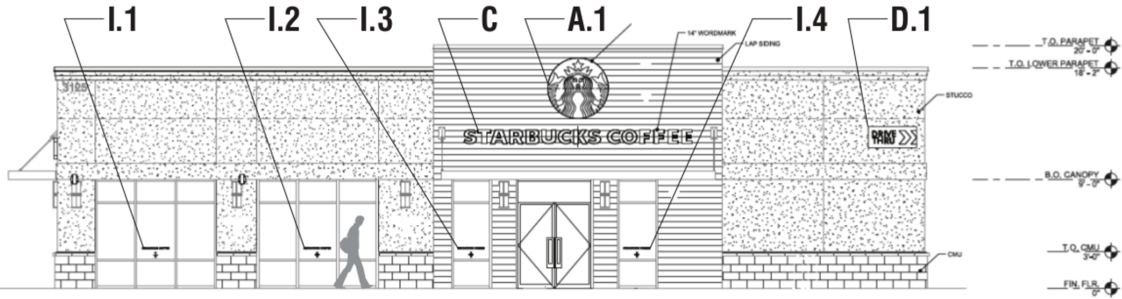
1 Elevation @ Main Entrance Approximate Scale: 1/8" = 1'-0"
