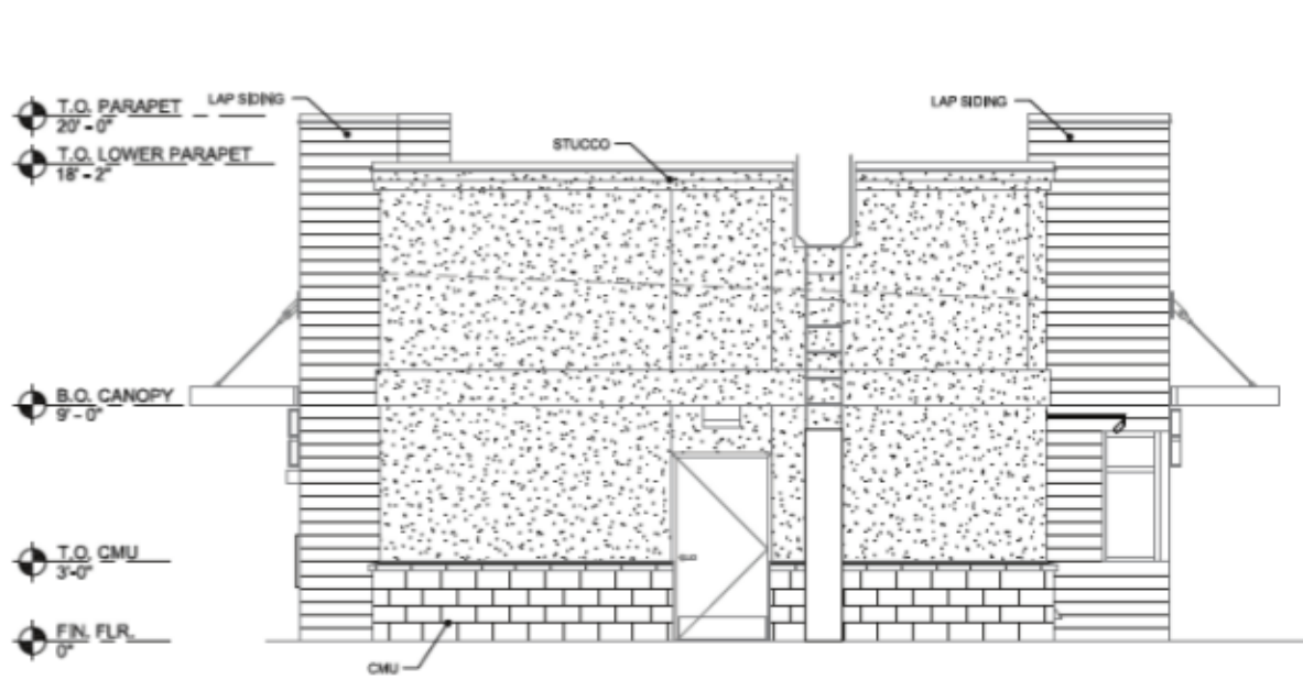
2 Elevation @ Back of House Approximate Scale: 1/8" = 1'-0"
